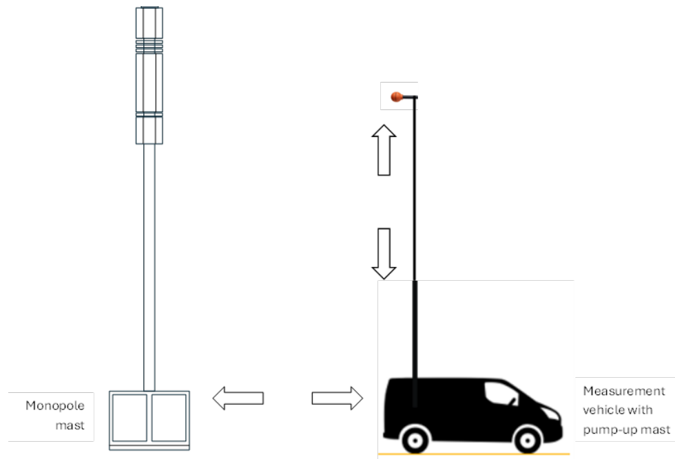
Figure 2: EMF measurement set-up
