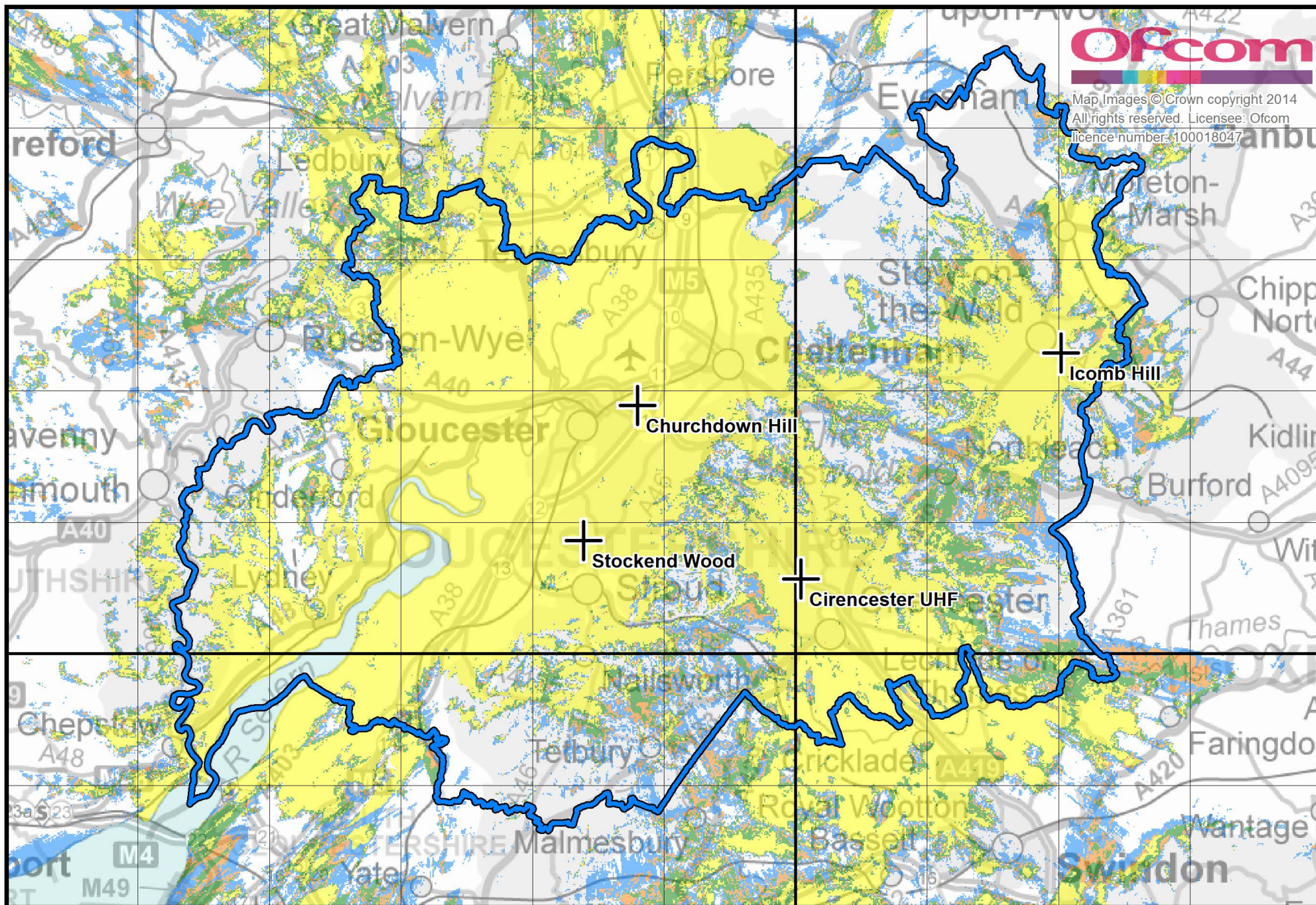
Gloucestershire Local DAB Multiplex Service Predicted mobile coverage enhanced propagation conditions, Final
