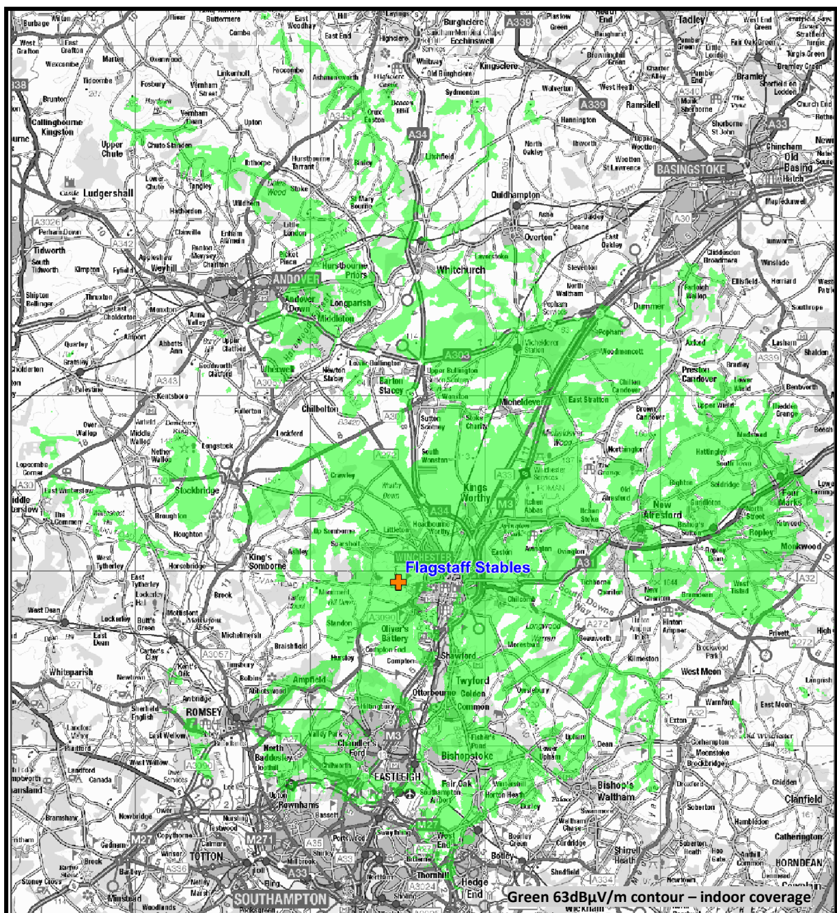
Figure 1: Predicted indoor coverage of the Winchester small-scale DAB multiplex. January 2024
